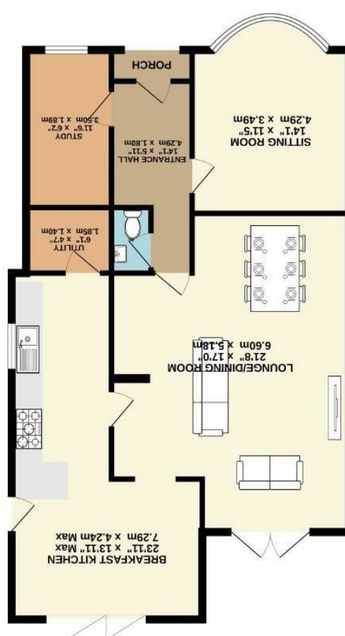
GROUND FLOOR 947 sq ft. (88.0 sq m.) approx.
